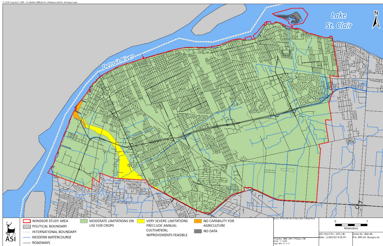
Figure A6: Soil Capability for Agriculture
